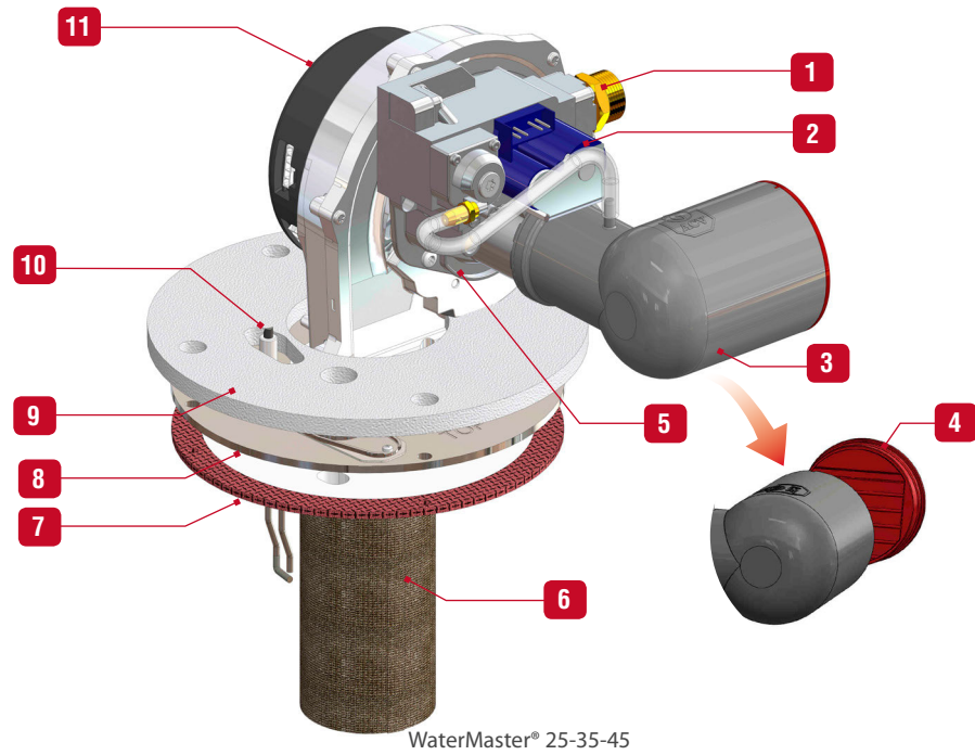
WaterMaster® 25-35-45
