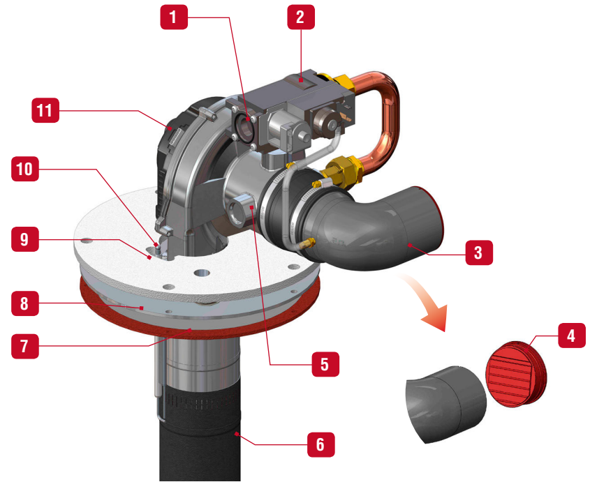
WaterMaster® 120
